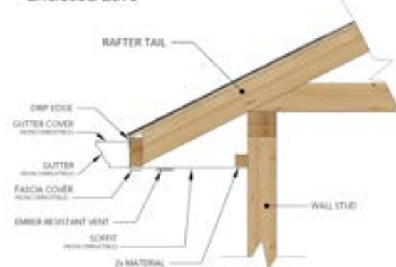
Enclosed Eave
